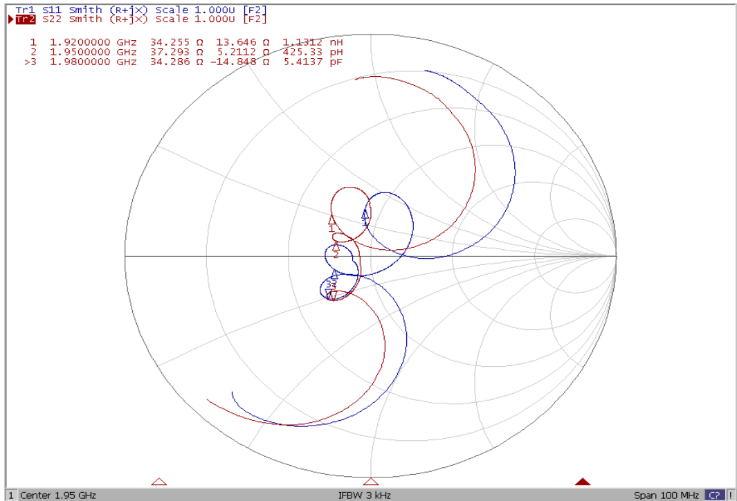
Smith Chart
